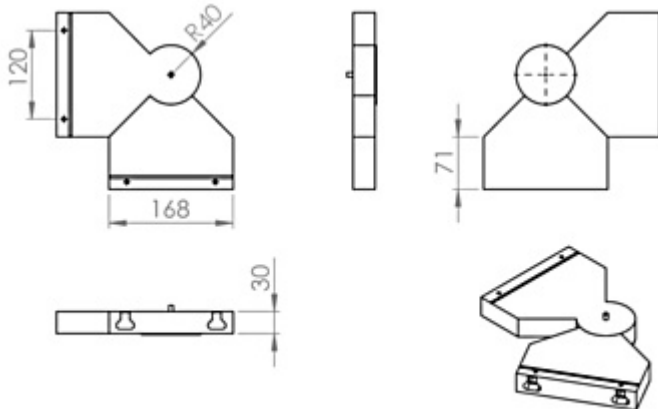
Sira Adjustable Corner
