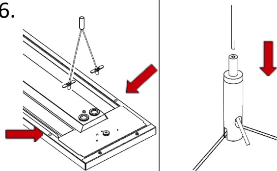
Insert toggles of Y suspension kit in to 7mm holes in luminaire
