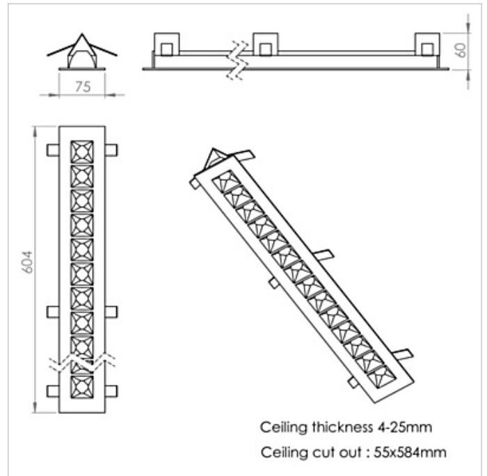
Rubini Recessed 600mm
