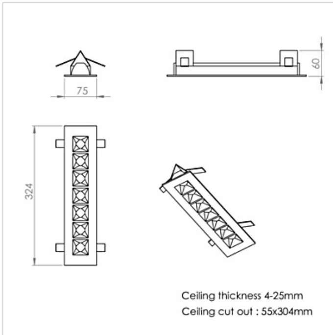
Rubini Recessed 300mm
