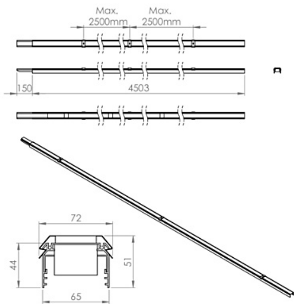
4500mm Trunking
