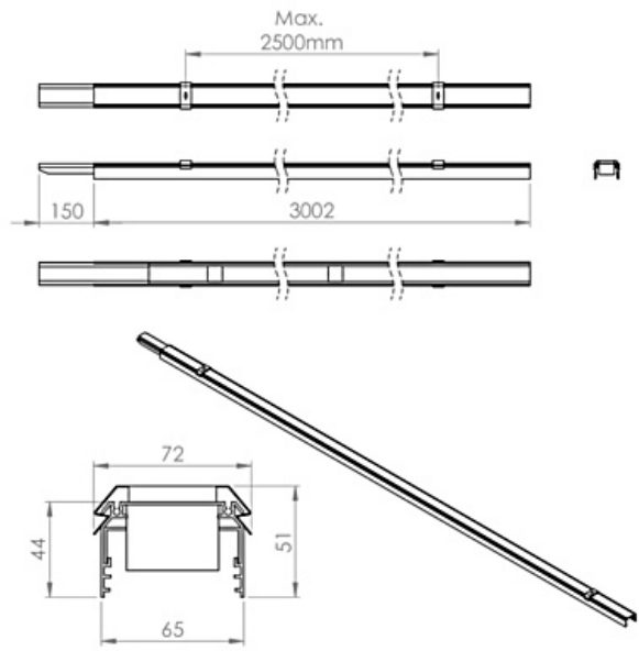
3000mm Trunking
