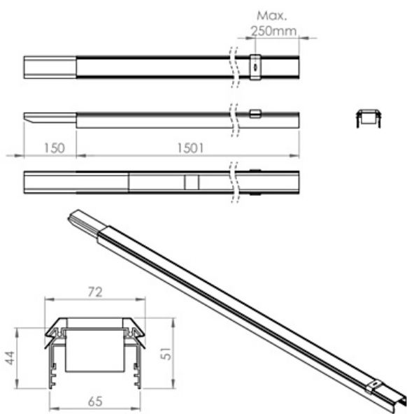
1500mm Trunking
