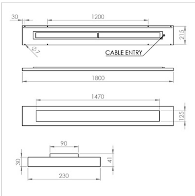
Element 1800mm
