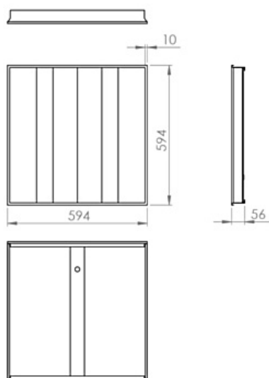
Arcus Duo Lay-In 600x600
