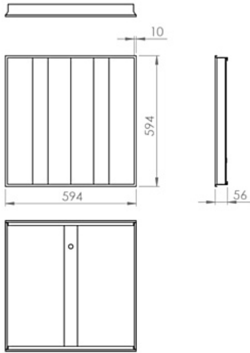
Arcus Duo Lay-In 600x600
