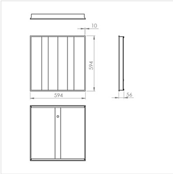
Arcus Duo Lay-In 600x600
