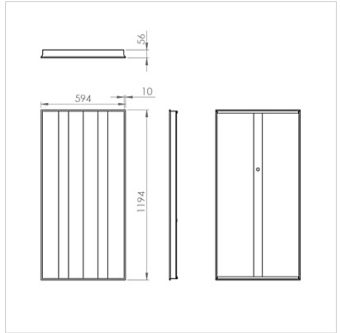
Arcus Duo Lay-In 1200x600
